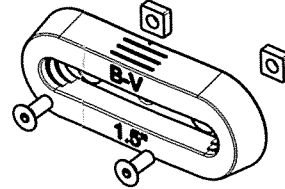
D020053(2SETS) L80XW31XTH.12mm
