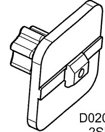
D020055(2SETS) L132XW31XTH.12mm
