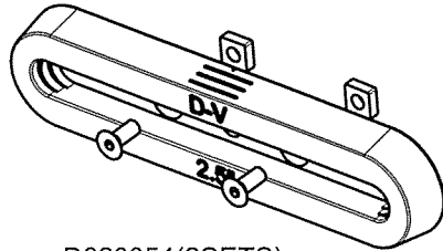
D020054(2SETS) L132XW31XTH.12mm
