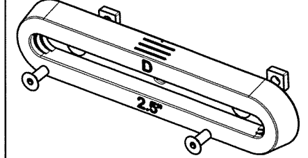
D020055(2SETS) L132XW31XTH.12mm
